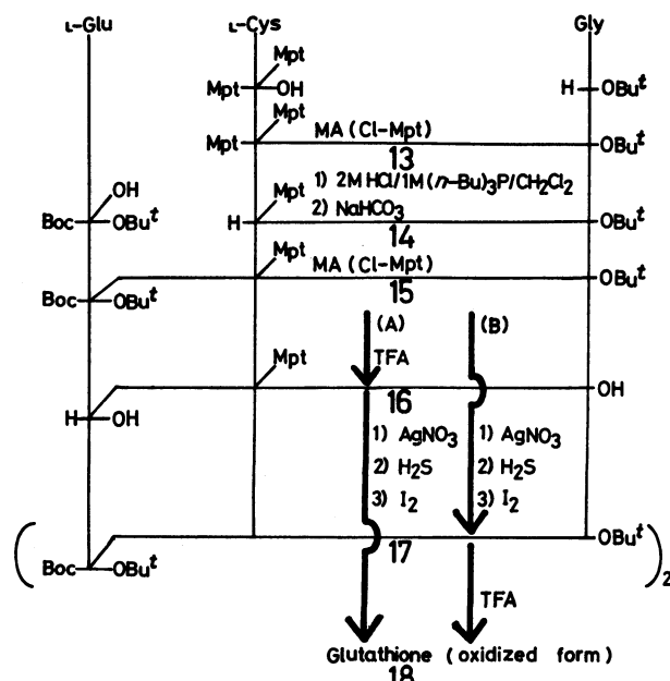
Fig. 4. Synthesis of glutathione.
