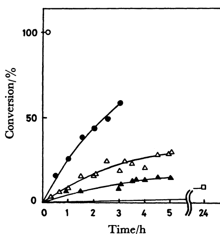
Fig. 1. Effects of the structure of tertiary amines on the dehydroalanine formation
