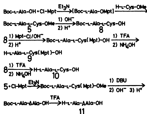
Fig. 2. Synthesis of model peptides.
